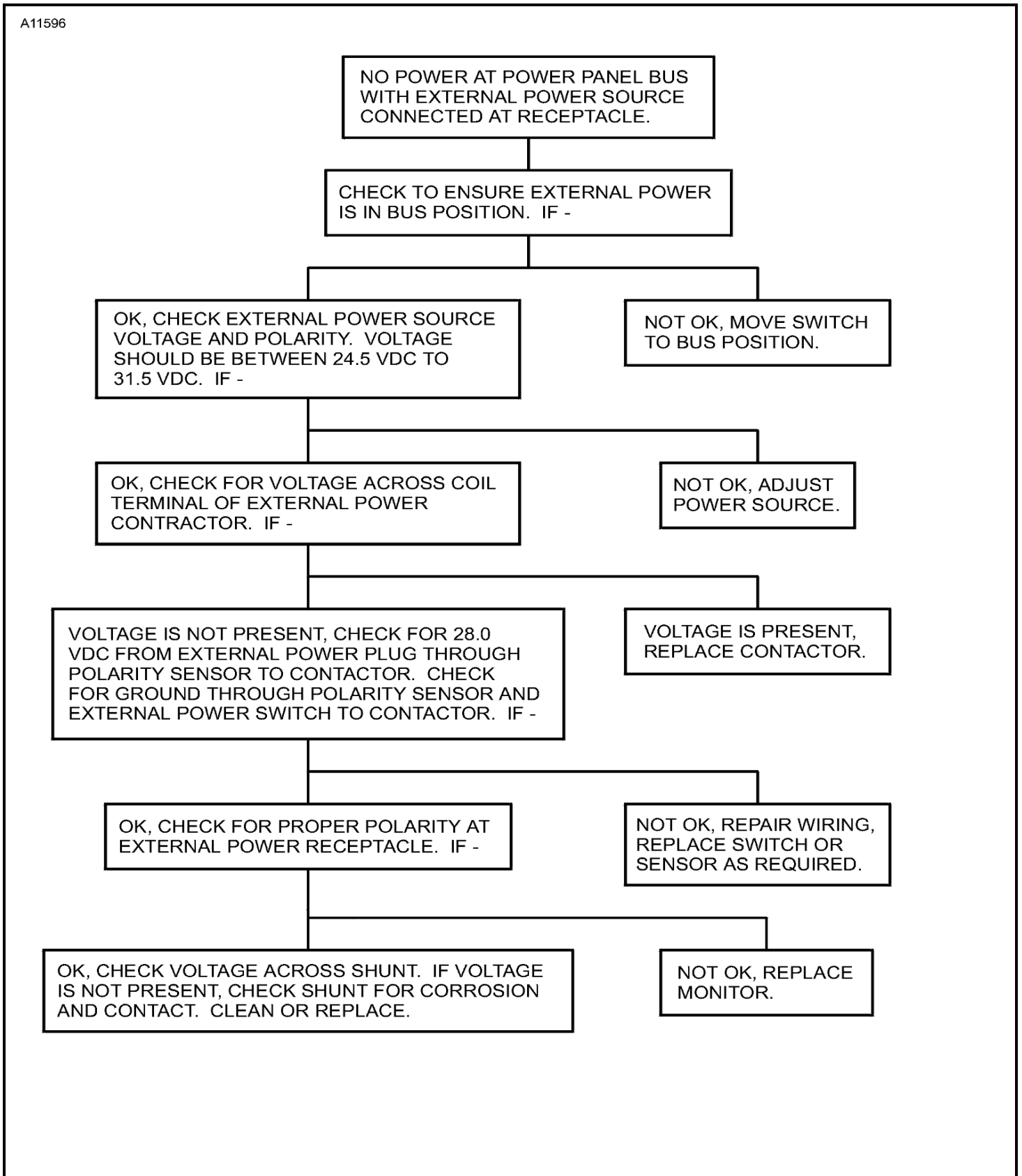
Figure 101 : Sheet 1 : External Power Troubleshooting Chart
